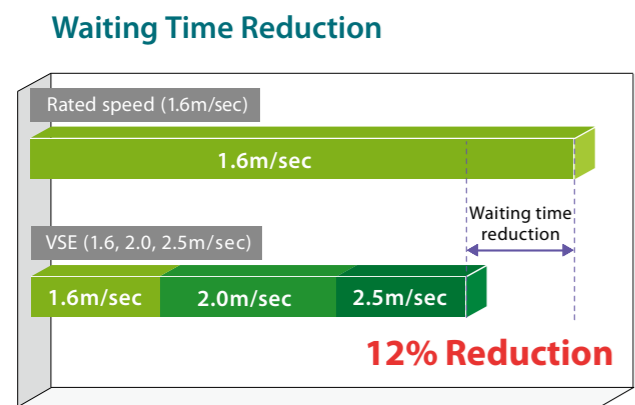
According to Mitsubishi Electric's simulation, waiting time can be reduced up to approximately 12% when VSE is applied.
